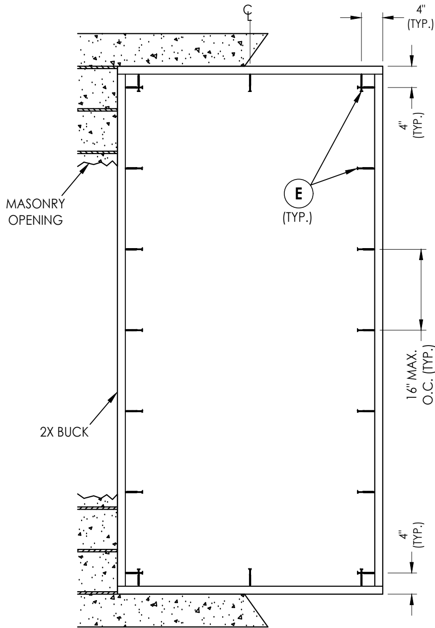
BUCK ANCHORING
