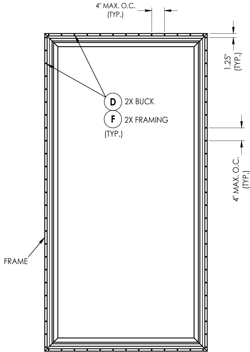
FRAME ANCHORING
